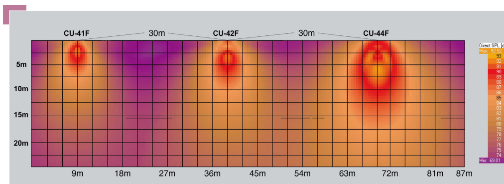
<Figure 2. CU-44F Horizontal simulation (2kHz)> * Scale Hight : 3m interval Width : 2.5m interval
