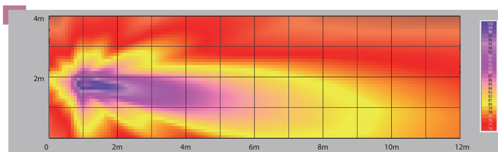
<Figure 1. Simulation with CU-44F viewed vertically (2kHz)> * Scale: 1m interval
