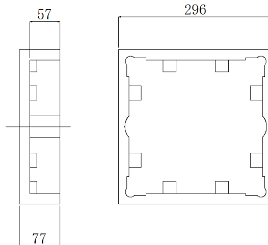
Pearl cotton box (unit: mm)
