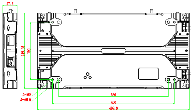
500×250mm Cabinet
