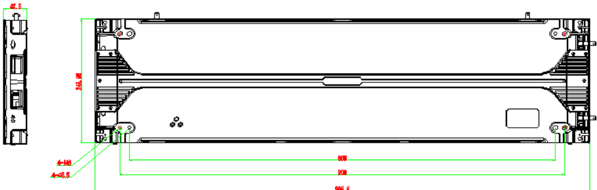
750×250mm Cabinet
