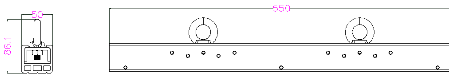
Hanging beam for 750*250mm cabinet (unit: mm)
