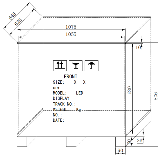
Module Carton and Wooden Box (unit: mm)
