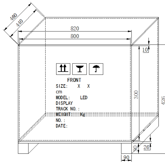
five in one wooden boxes (unit in the figure: mm)
