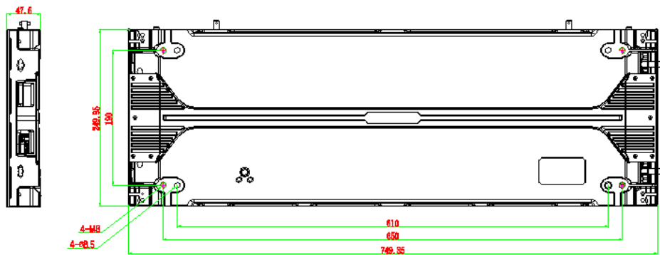
750×250mm Cabinet
