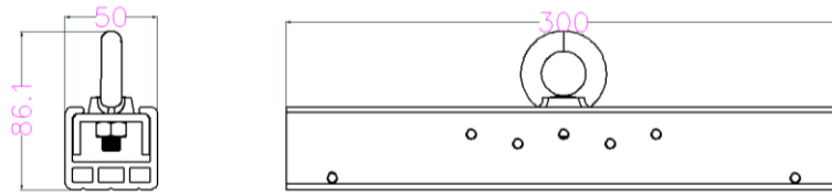
Hanging beam for 500*250mm cabinet (unit: mm)
